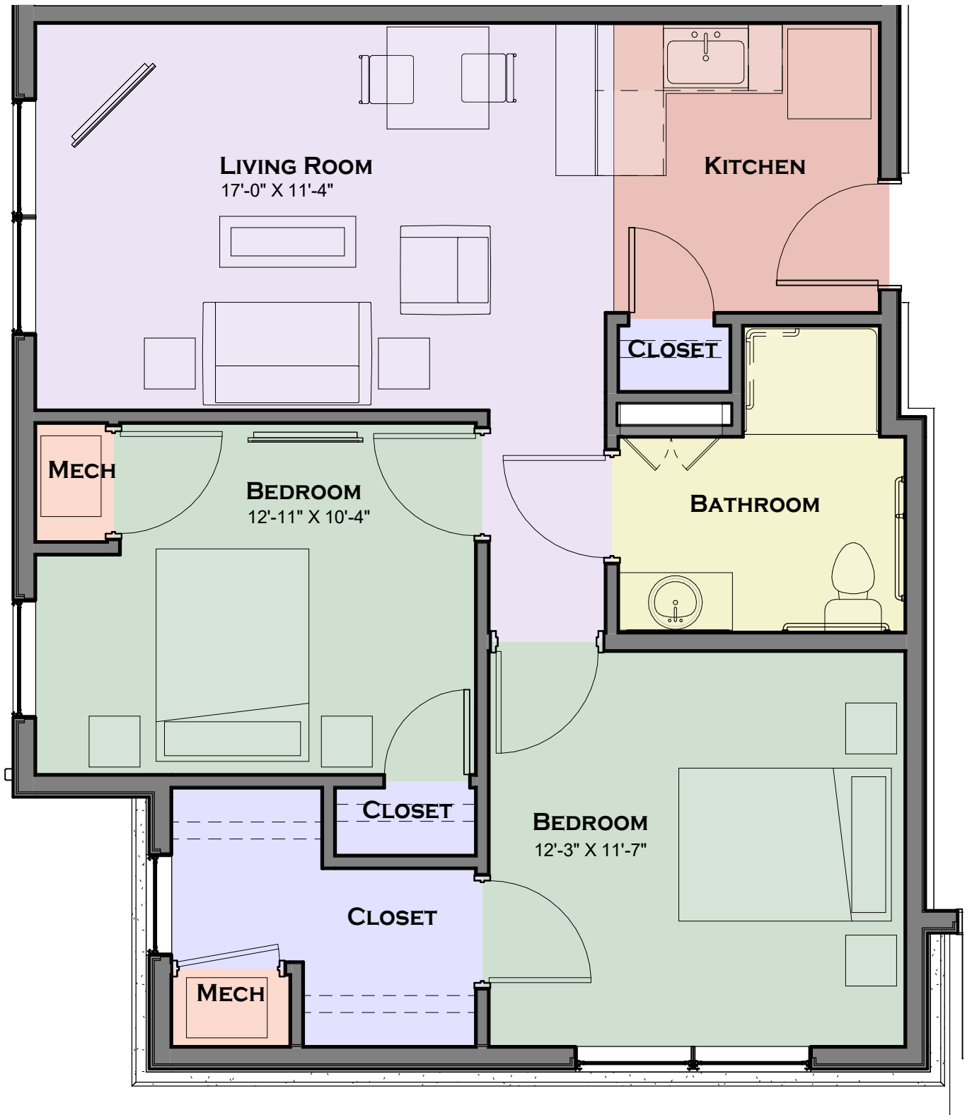
① UNIT J PLAN 764 SF 1/4" = 1'-0"
