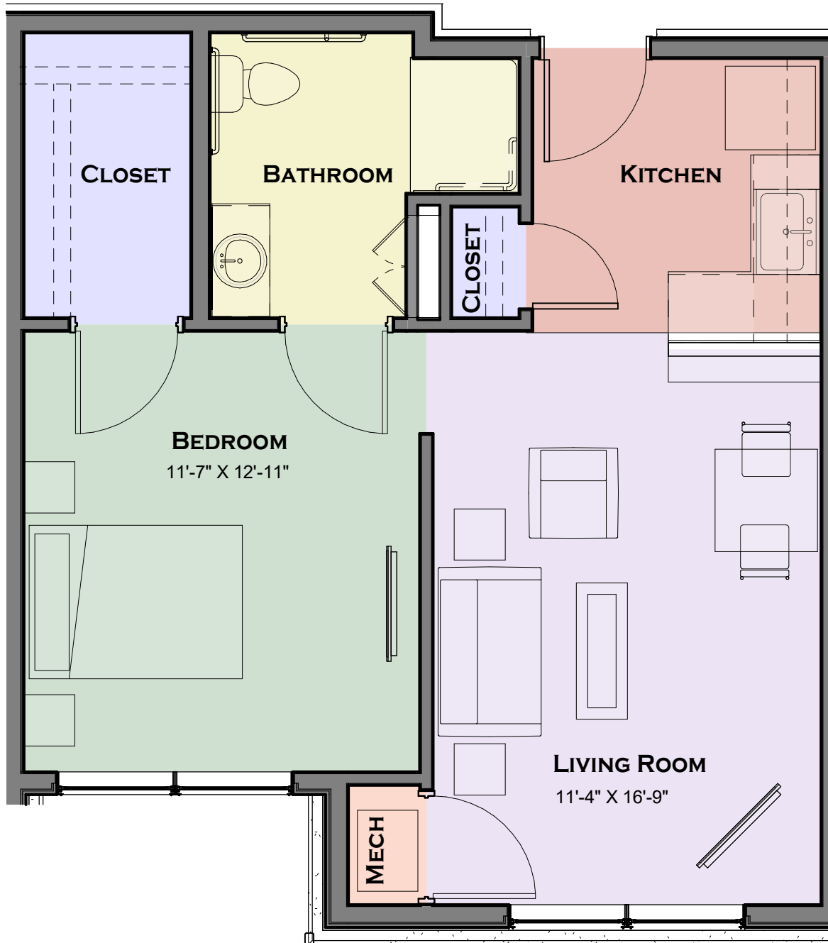
① UNIT D PLAN 582 SF 1/4" = 1'-0"
